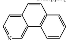
Benzo[h]isoquinoline
