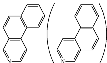
Benzo[f]isoquinoline
