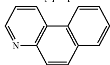
Benzo[f]quinoline
