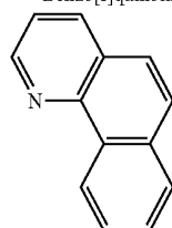
Benzo[h]quinoline
